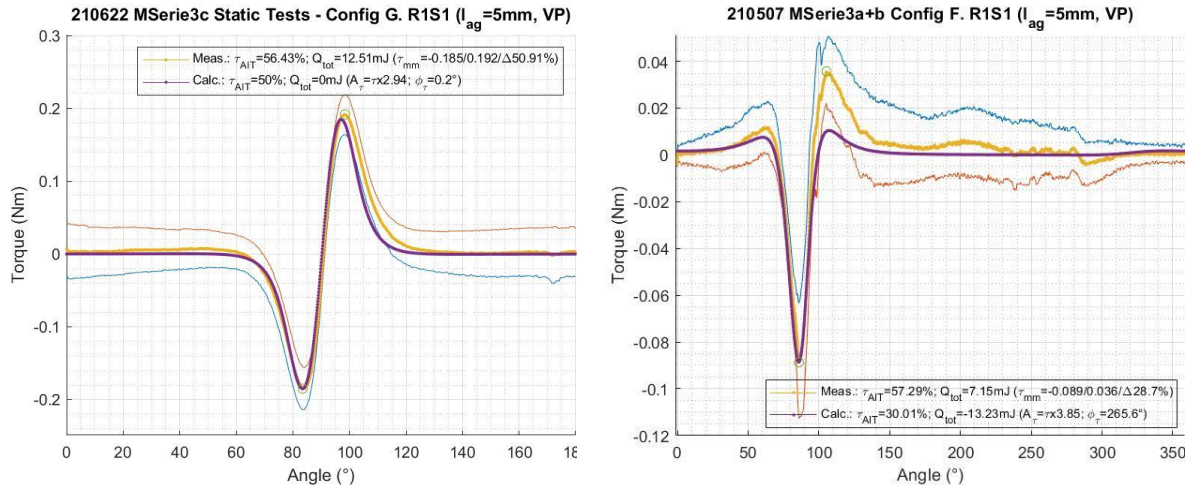
Fig. 16. Static torque signals: sym. commensurable torque reference (lhs) created by config. 03.G and asym. incommensurable torque (rhs) created by config 03.F – compare Fig. 10 and Fig. 11
