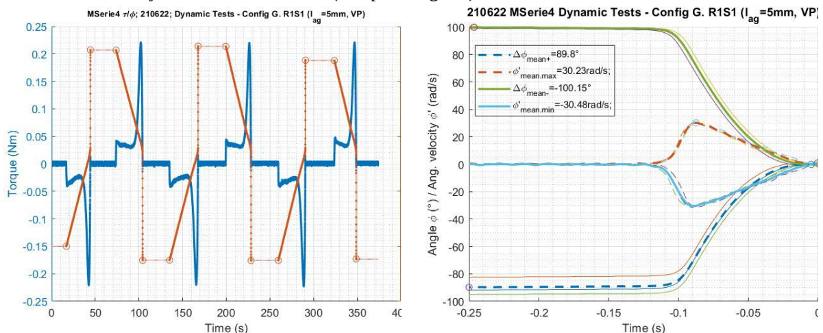
Fig. 17. Validation of a symmetric commensurable torque signal, for reference test purposes – also compare config. 03.G in Fig. 10 and Fig. 11
