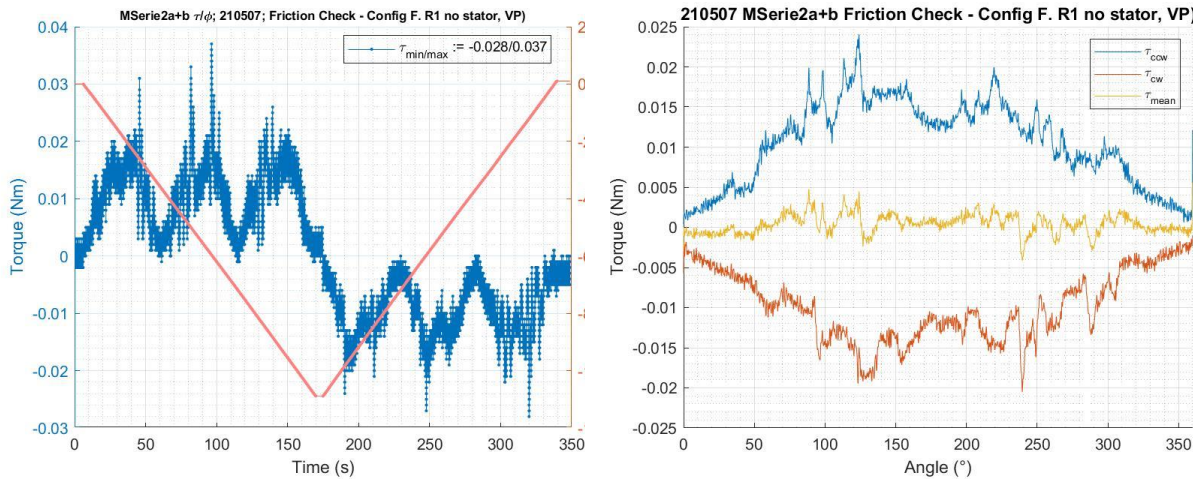
Fig. 15. Friction signals, raw data (lhs) and 3x superposed friction signal (rhs)
