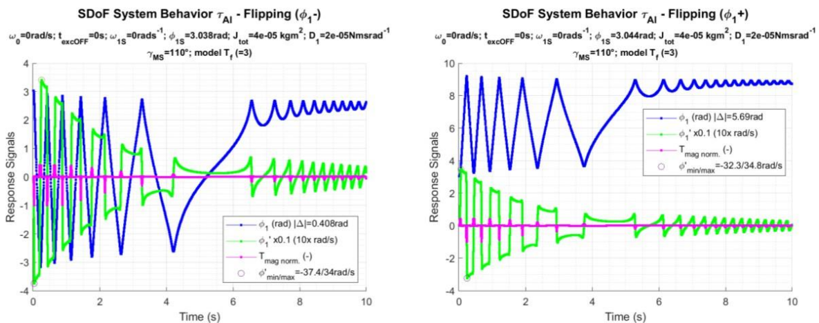
Fig. 25. Nonlinear asymmetric incommensurable torque spring \tau_{AI} behavior
