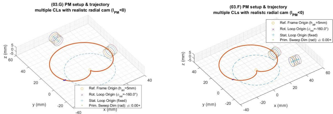
Fig. 10. Setup of circular stator and rotor PM structures and symmetric placed stator (config. 03.G, lhs) and an asymmetric placed stator (config. 03.F, rhs) with the same cam trajectory (in red); cam parameters in Table 3
