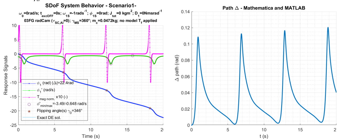
Fig. 21. Comparison of resulting trajectories no damping and no stiffness applied. Initial conditions: \phi(0) = 0 and \phi'(0) = -1 \text{ rad/s} (lhr); path error of exact and approx. solution (rhs)
