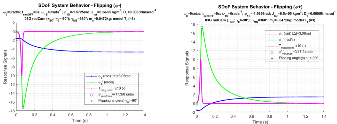
Fig. 12. Nonlinear symmetric commensurable torque spring in config. 03.G (see Fig. 10, lhs)
