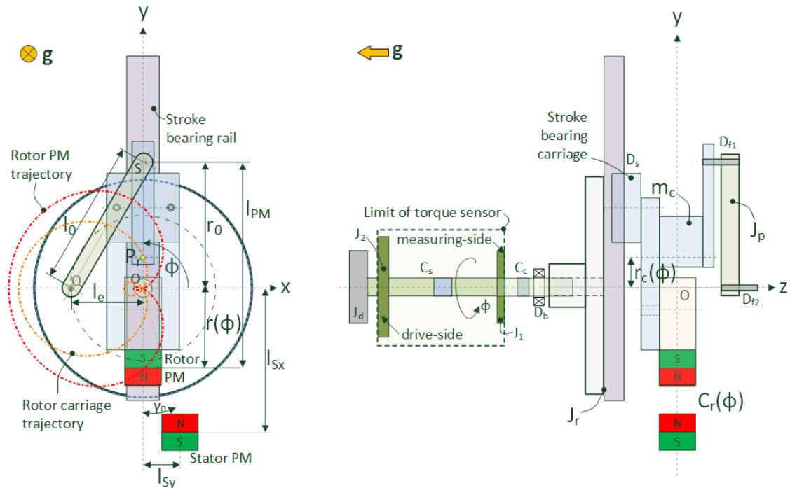
Fig. 5. Lumped parameter model in ground view (lhs) and profile (rhs)
