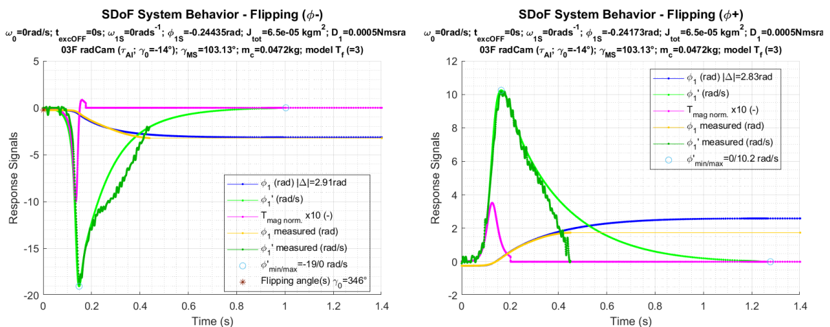
Fig. 19. Validation of an AIT signal in config. 03.F (setup shown in Fig. 10, rhs)
