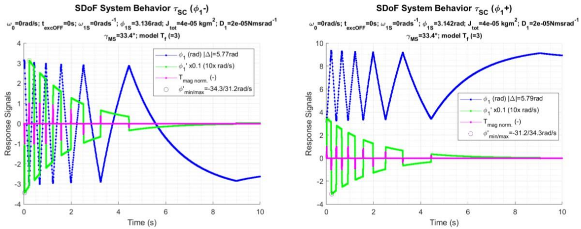
Fig. 23. Nonlinear symmetric commensurable torque spring \tau_{SC} behavior
