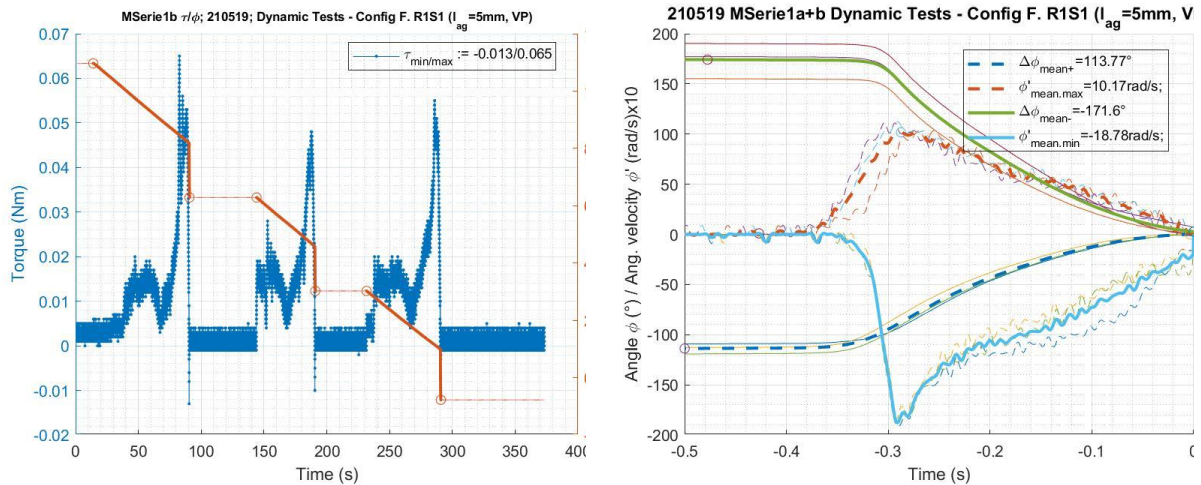
Fig. 18. Validation of an AIT signal– also compare config. 03.F in Fig. 10 and Fig. 11
