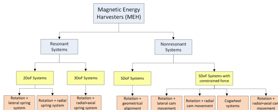
Fig. 2. Classification of MEH systems
