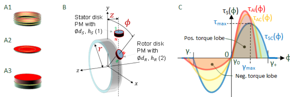
Fig. 1. PM modeling by means of current loops (shown in yellow, A1-3, lhs). Revolving rotor with disk PM's (in the middle, B). On rhs, C, generated torque signals due to nonlin. EM springs
