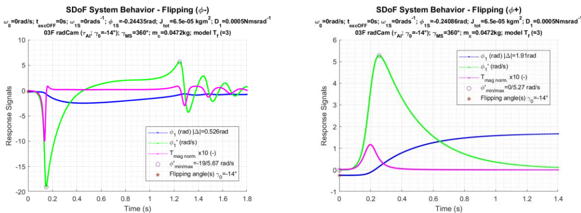
Fig. 13. Nonlinear asymmetric incommensurable torque spring in config 03.F (see Fig. 10, rhs)
