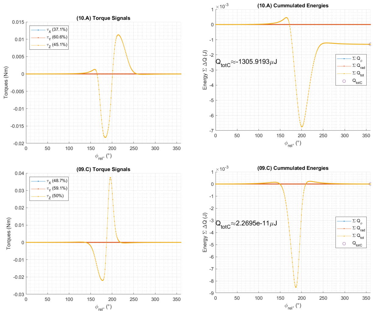
Fig. 8. Calculated torque (lhs) on rotor and energies (rhs) for shown setups in Fig. 7
