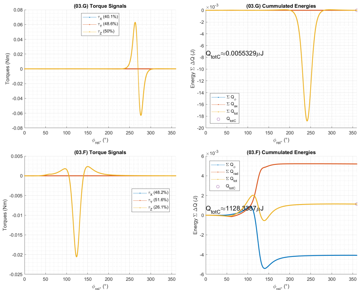
Fig. 11. Calculated torque (lhs) on rotor and energies (rhs) for setups shown in Fig. 10 (lhs and rhs)
