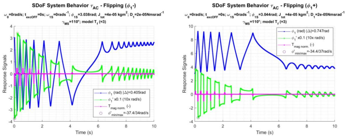
Fig. 24. Nonlinear asymmetric commensurable torque spring \tau_{AC} behavior
