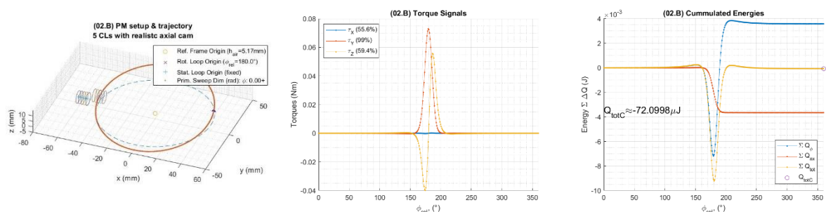
Fig. 9. PM setup of with circular shells of stator and rotor and an asymmetric placed cam trajectory (in red) with cam parameters shown in Table 2 (lhs); calculated torque (middle) and energies (rhs)
